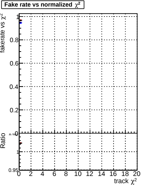
Fake rate vs. DOM original DOM firstTest byPassRefit DOM firstTestFit 1000ev
