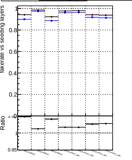
Fake rate vs. DOM original DOM firstTest byPassRefit DOM firstTestFit 1000ev
