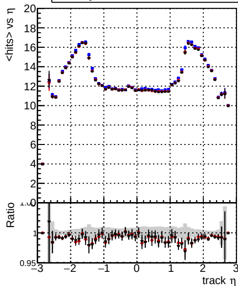
mean hits vs \eta — DQM_original — DQM_firstTest_byPassRefit — DQM_firstTestFit4_1000ev
