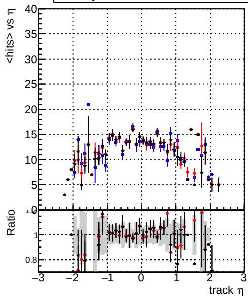
mean hits vs \eta — DQM_original — DQM_firstTest_byPassRefit — DQM_firstTestFit4_1000ev
