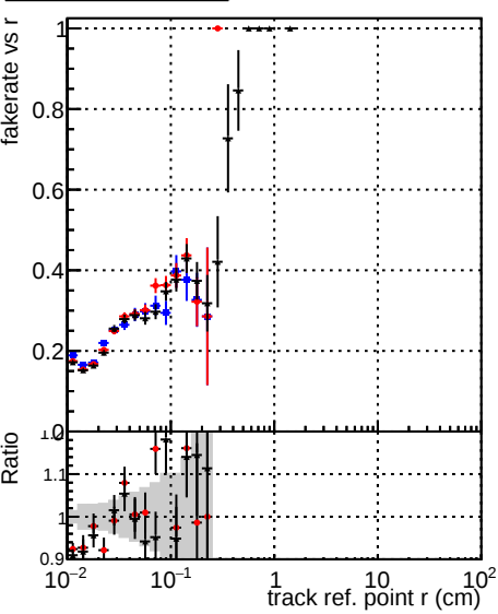
Fake rate vs v Legend: DQM_original (blue line with circles) DQM_firstTest_byPassRefit (red line with circles) DQM_firstTestFit4_1000ev (black line with circles)
