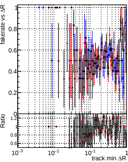
Legend: DQM original (blue), DQM firstTest byPassRefit (red), DQM firstTestFit4_1000ev (black)
