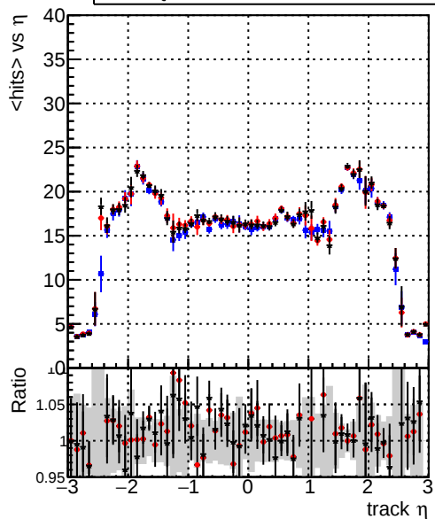
mean hit — DQM_original — DQM_firstTest_byPassRefit — DQM_firstTestFit4_1000ev
