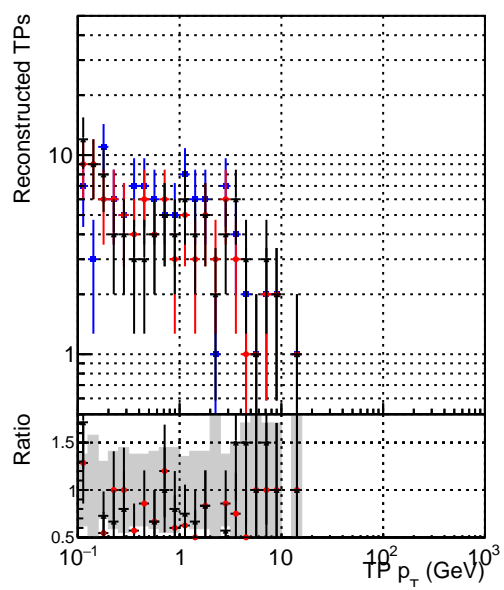
Legend: DQM_original (blue circle), DQM_firstTest_byPassRefit (red circle), DQM_firstTestFit4_1000ev (black star)
