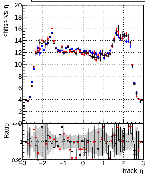
DQM_original DQM_firstTest_byPassRefit DQM_firstTestFit4_1000ev mean hits
