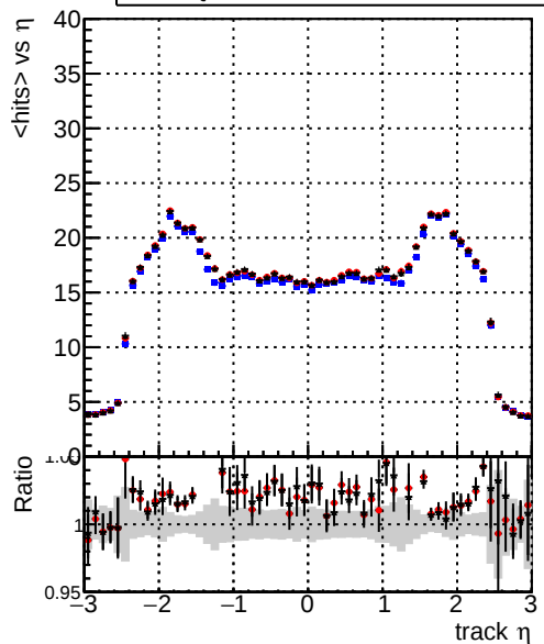
mean hits — DQM_original — DQM_firstTest_byPassRefit — DQM_firstTestFit4_1000ev
