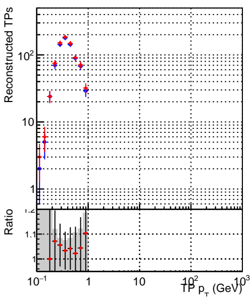
■ DQM_original ■ DQM_firstTest_byPassRefit
