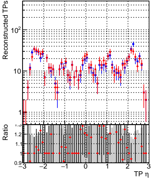
■ DQM_original ■ DQM_firstTest_byPassRefit
