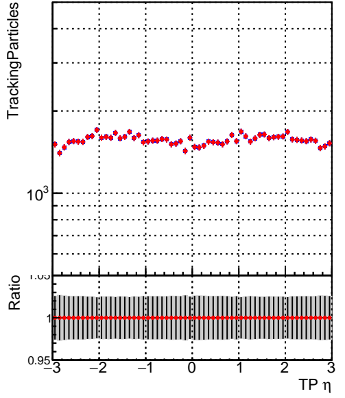
■ DQM_original ■ DQM_firstTest_byPassRefit
