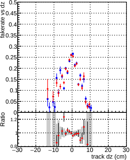
Fake rate vs dz DQM_original DQM_firstTest_byPassRefit
