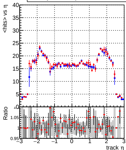
mean hits vs \eta Legend: DQM_original (blue line), DQM_firstTest_byPassRefit (red line)
