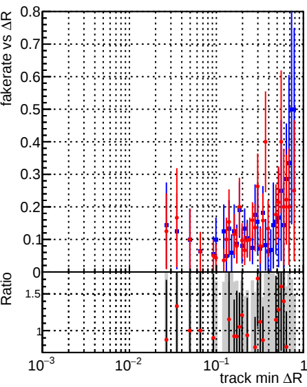
Fake rate vs ΔR(track, jet) DQM_original DQM_firstTest_byPassRefit
