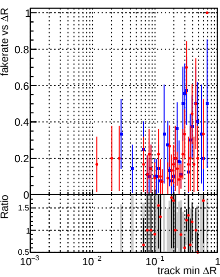
Fake rate vs \Delta R(\text{track, jet}) DQM_original DQM_firstTest_byPassRefit
