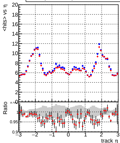
mean hits — DQM_original — DQM_firstTest_byPassRefit
