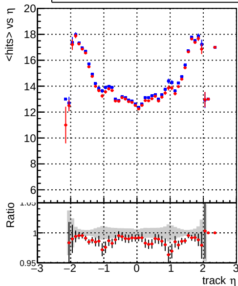
mean hits vs \eta — DQM_original — DQM_firstTest_byPassRefit
