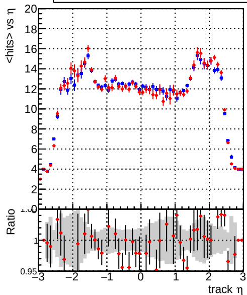
mean hit — DQM_original — DQM_firstTest_byPassRefit
