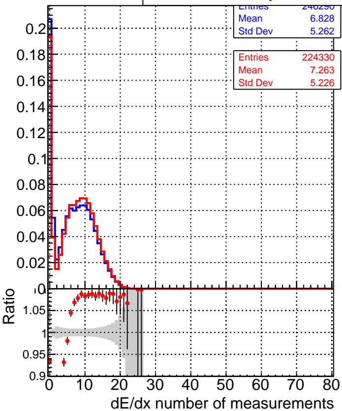
■ DQM_original ● DQM_firstTest_byPassRefit
