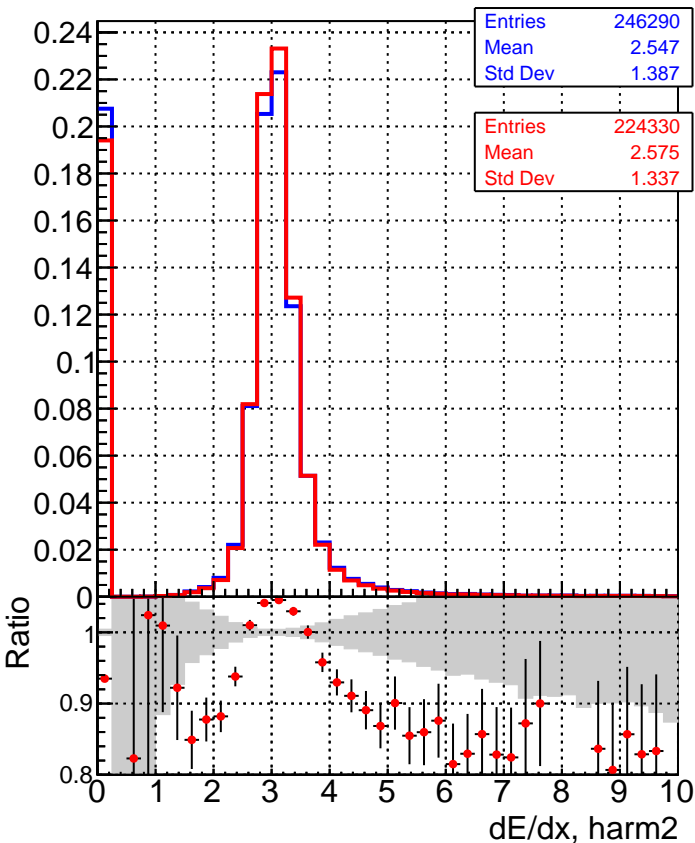
■ DQM_original ● DQM_firstTest_byPassRefit
