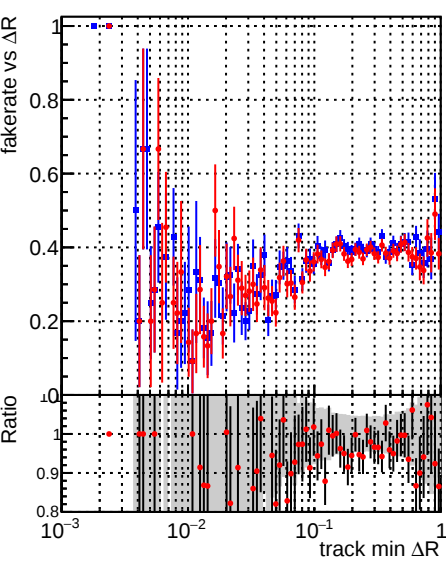
Fake rate vs \Delta R (track, jet) DQM_original DQM_firstTest_byPassRefit
