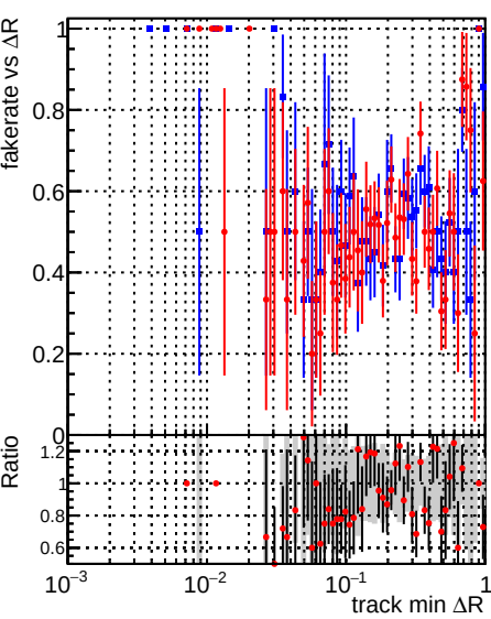
Fake rate vs \Delta R(\text{track, jet}) Legend: —■— DQM_original —■— DQM_firstTest_byPassRefit
