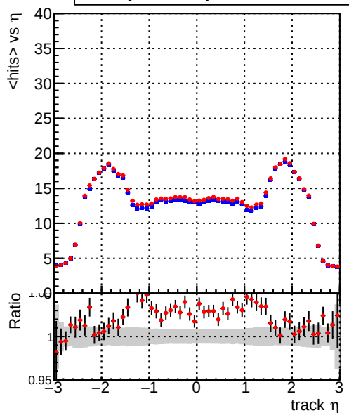
mean hits vs \eta — DQM_original — DQM_firstTest_byPassRefit
