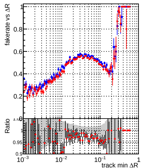
Fake rate vs \Delta R (track, jet) Legend: —•— DQM_original —•— DQM_firstTest_byPassRefit
