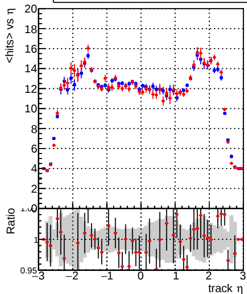
mean hits vs \eta Legend: — DQM_original, — DQM_firstTest_byPassRefit
