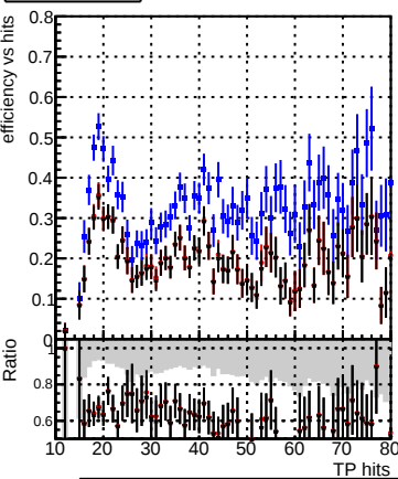
Efficiency vs hit Legend: DQM_original4_step2_pt0p1to1_eta0p0to0p4 DQM_testMkFit_step2_pt0p1to1_eta0p0to0p4 DQM_testMkFit_step2_pt0p1to1_eta0p0to0p4_testX
