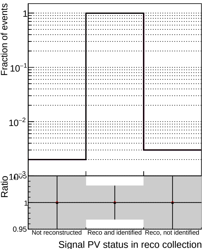
TruePVLocationIndexInRecoVertexCollectionCumulative
