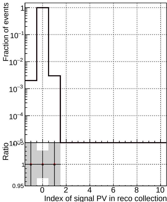
TruePVLocationIndexInRecoVertexCollection
