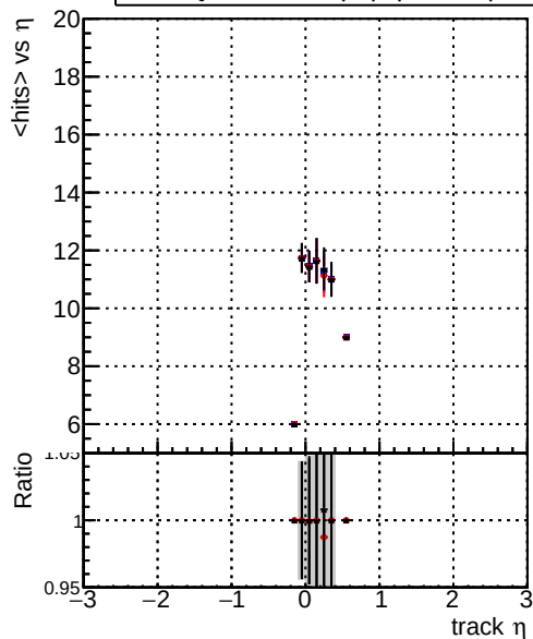
mean hits — DQM_original4_step2_pt0p1to1_eta0p0to0p4 — DQM_testMkFit_step2_pt0p1to1_eta0p0to0p4 — DQM_testMkFit_step2_pt0p1to1_eta0p0to0p4_testx
