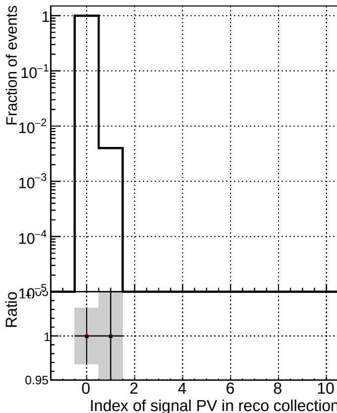
TruePVLocationIndexInRecoVertexCollection
