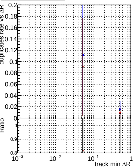
Legend: - blue line with dots: DQM_original4_step2_pt0p1to1_eta0p0to0p4 - red line with dots: DQM_testMkFit_step2_pt0p1to1_eta0p0to0p4 - black line with dots: DQM_testMkFit_step2_pt0p1to1_eta0p0to0p4_testX
