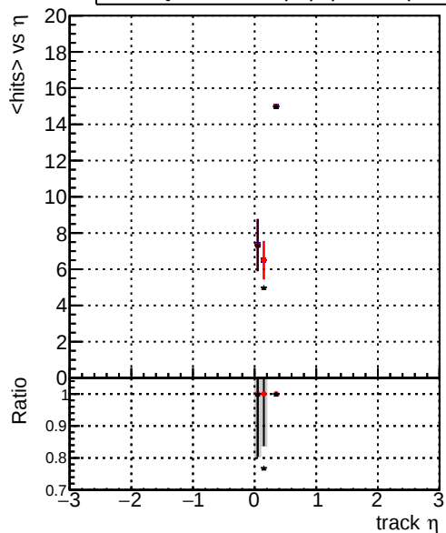
mean hits — DQM_original4_step2_pt0p1to1_eta0p0to0p4 — DQM_testMkFit_step2_pt0p1to1_eta0p0to0p4 — DQM_testMkFit_step2_pt0p1to1_eta0p0to0p4_testx
