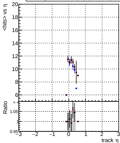
mean hit — DQM_original4_step2_pt0p1to1_eta0p0to0p4 — DQM_testMkFit_step2_pt0p1to1_eta0p0to0p4 — DQM_testMkFit_step2_pt0p1to1_eta0p0to0p4_testx
