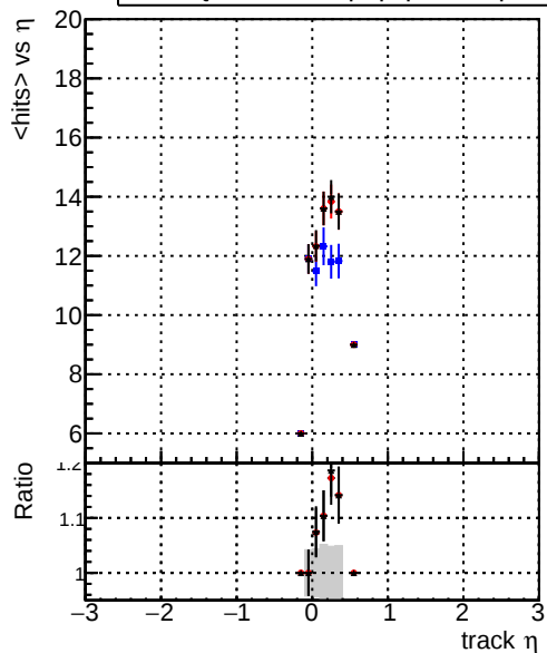
— DQM_original4_step2_pt0p1to1_eta0p0to0p4 — DQM_testMkFit_step2_pt0p1to1_eta0p0to0p4 — DQM_testMkFit_step2_pt0p1to1_eta0p0to0p4_testx
