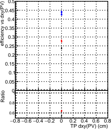
Efficiency vs Dxy(PV) Legend: DQM_original4_step2_pt0p1to1_eta2p0to2p5 DQM_testMkFit_step2_pt0p1to1_eta2p0to2p5 DQM_testMkFit_step2_pt0p1to1_eta2p0to2p5_testX
