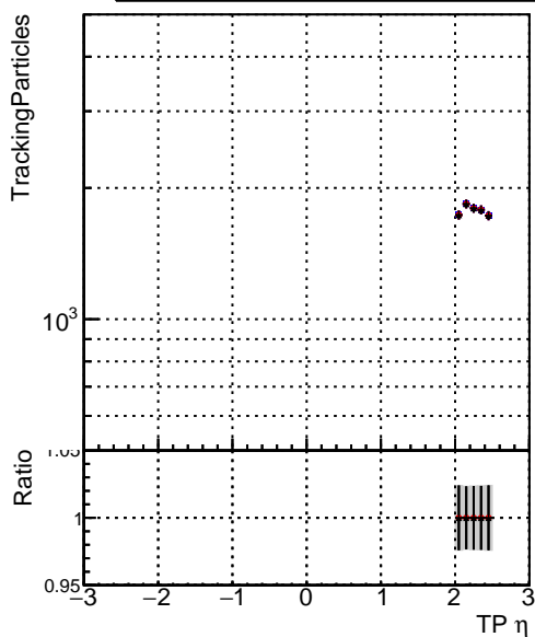
N of sin —●— DQM_testMkFit_step2_pt0p1to1_eta2p0to2p5 —▲— DQM_testMkFit_step2_pt0p1to1_eta2p0to2p5_testX
