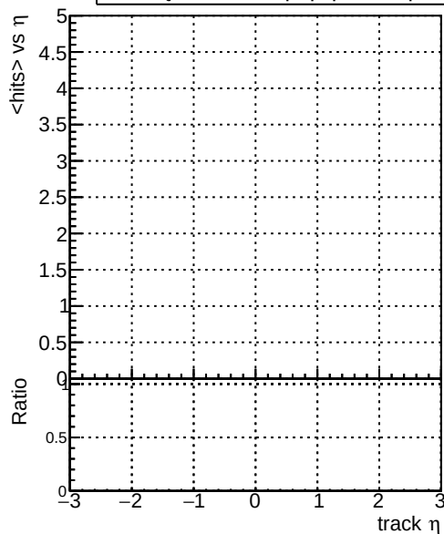
— DQM_original4_step2_pt0p1to1_eta2p0to2p5 — DQM_testMkFit_step2_pt0p1to1_eta2p0to2p5 — DQM_testMkFit_step2_pt0p1to1_eta2p0to2p5_testx
