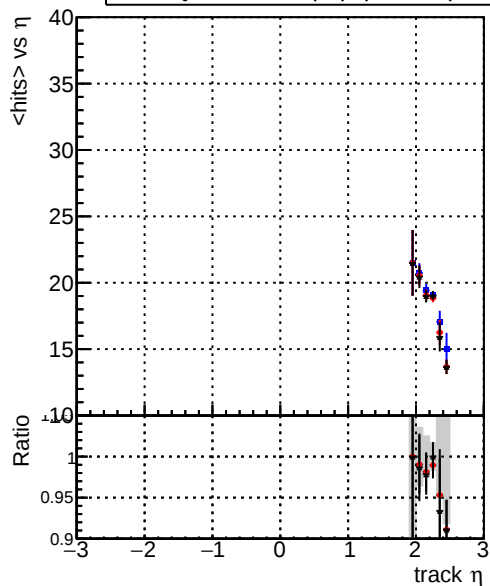
mean hits — DQM_original4_step2_pt0p1to1_eta2p0to2p5 — DQM_testMkFit_step2_pt0p1to1_eta2p0to2p5 — DQM_testMkFit_step2_pt0p1to1_eta2p0to2p5_testx
