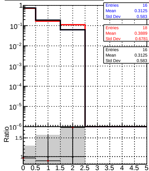
mean hit — DQM_original4_step2_pt0p1to1_eta2p0to2p5 — DQM_testMkFit_step2_pt0p1to1_eta2p0to2p5 — DQM_testMkFit_step2_pt0p1to1_eta2p0to2p5_testx
