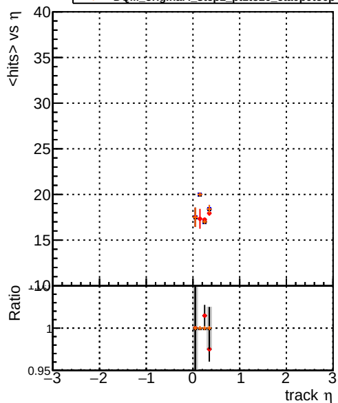
mean hits DQM_original4_step2_pt1to20_eta0p0to0p4 DQM_testMkFitFit_step2_pt1to20_eta0p0to0p4_sl100 DQM_original4_step2_pt1to20_eta0p0to0p4_simplerCPE DQM_original4_step2_pt1to20_eta0p0to0p4_simplerCPE2
