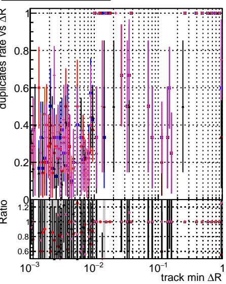
— DOM original_step2_pt1to20_eta0p0to0p4 — last_step2_pt1to20_eta0p0to0p4 — last_step2_pt1to20_eta0p0to0p4 — CE Pixel3 Step2_pt1to20_eta0p0to0p4
