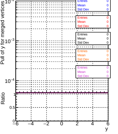
RecoAllAssoc2GenMatchedMerged_PullY
