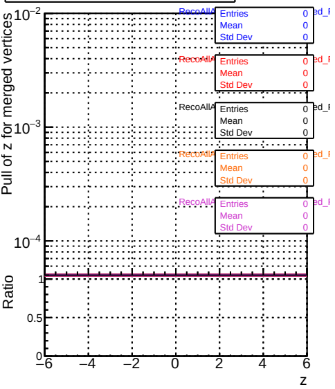
RecoAllAssoc2GenMatchedMerged_PullZ
