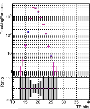
— DQM_original_step2_pt1to20_eta0p0to0p4 — DQM_angle_step2_pt1to20_eta0p0to0p4 — DQM_mkFit_step2_pt1to20_eta0p0to0p4 — DQM_mkFit_step2_pt1to20_eta0p0to0p4 — DQM_CPEpixel3_step2_pt1to20_eta0p0to0p4
