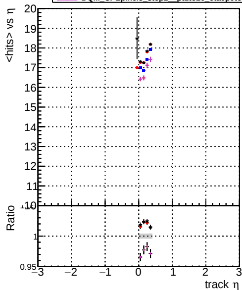
mean hit DOM original_step2_pt1to20_eta0p0to0p4 DOM angle_step2_pt1to20_eta0p0to0p4 DOM fast_step2_pt1to20_eta0p0to0p4 DOM mkFit_step2_pt1to20_eta0p0to0p4 DOM CPEpixel3_step2_pt1to20_eta0p0to0p4
