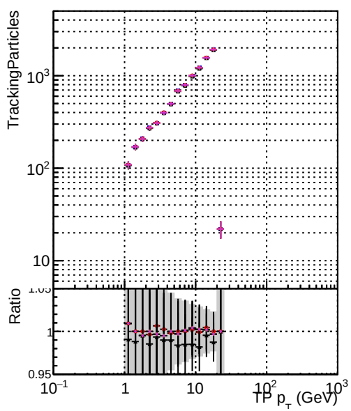
— DQM original_step2_pt1to20_eta0p0to0p4 — DQM angle_step2_pt1to20_eta0p0to0p4 — DQM fast_step2_pt1to20_eta0p0to0p4 — DQM mkFit_step2_pt1to20_eta0p0to0p4 — DQM CPEpixel3_step2_pt1to20_eta0p0to0p4
