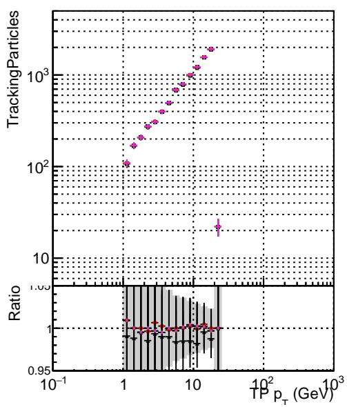
— DQM_original_step2_pt1to20_eta0p0to0p4 — DQM_angle_step2_pt1to20_eta0p0to0p4 — DQM_fast_step2_pt1to20_eta0p0to0p4 — DQM_mkFit_step2_pt1to20_eta0p0to0p4 — DQM_CPEpixel3_step2_pt1to20_eta0p0to0p4
