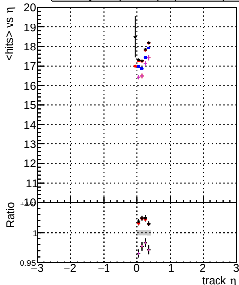
mean hit DOM original_step2_pt1to20_eta0p0to0p4 DOM angle_step2_pt1to20_eta0p0to0p4 DOM fast_step2_pt1to20_eta0p0to0p4 DOM mkFit_step2_pt1to20_eta0p0to0p4 DOM CPEpixel3_step2_pt1to20_eta0p0to0p4
