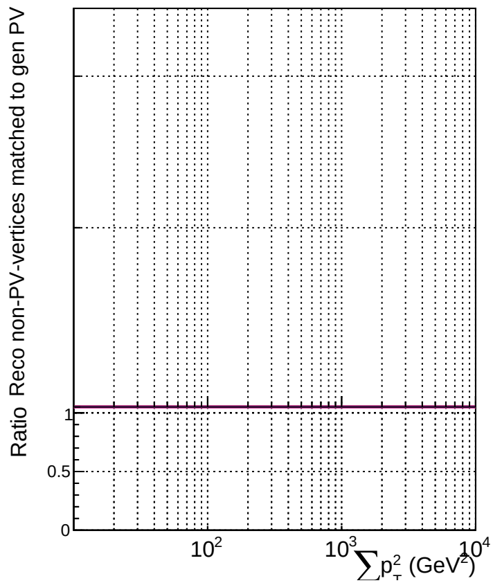
RecoAssoc2GenPVMatchedNotHighest_Pt2
