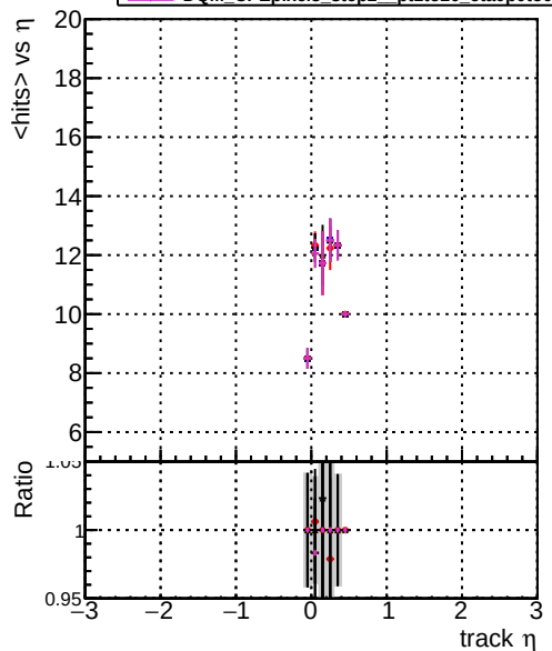
mean hits vs \eta Legend: DOM original step2 pt1to20 eta0p0to0p4 DOM angle step2 pt1to20 eta0p0to0p4 DOM fast step2 pt1to20 eta0p0to0p4 DOM mkFit step2 pt1to20 eta0p0to0p4 DOM CPEpixel3_step2_pt1to20_eta0p0to0p4
