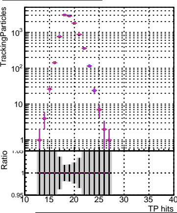
— DQM_original_step2_pt1to20_eta0p0to0p4 — DQM_angle_step2_pt1to20_eta0p0to0p4 — DQM_mkFit_step2_pt1to20_eta0p0to0p4 — DQM_mkFit_step2_pt1to20_eta0p0to0p4 — DQM_CPEpixel3_step2_pt1to20_eta0p0to0p4
