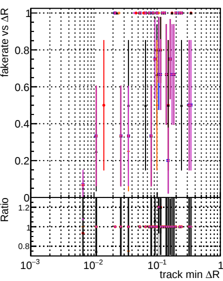
Fake rate vs \Delta R(\text{track, jet}) DOM original_step2 pt1to20_eta0p0to0p4 fixed_step2 last_step2 pt1to20_eta0p0to0p4 CLEF
