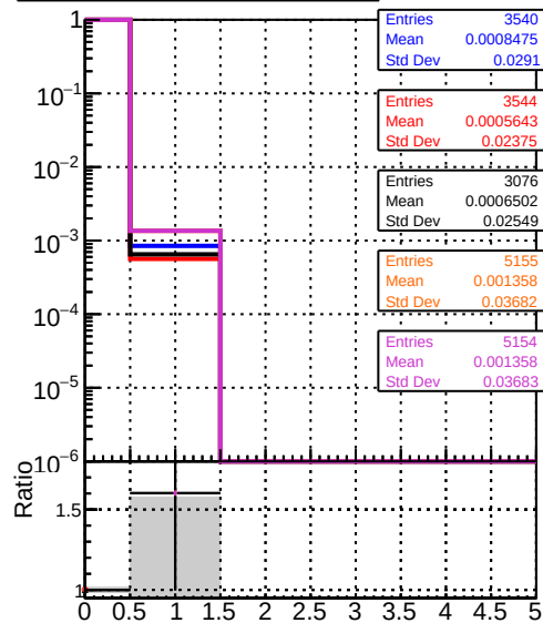
Legend for mean hits vs \eta : DOM original step2_pt1to20_eta0p0to0p4 DOM angle_step2_pt1to20_eta0p0to0p4 DOM fast_step2_pt1to20_eta0p0to0p4 DOM mkFit_step2_pt1to20_eta0p0to0p4 DOM CPEpixel2_step2_pt1to20_eta0p0to0p4
