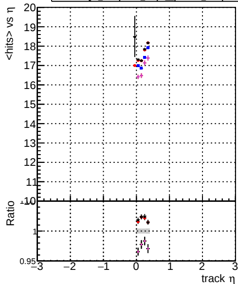
Legend for mean hits vs \eta : DOM original step2_pt1to20_eta0p0to0p4 DOM angle_step2_pt1to20_eta0p0to0p4 DOM fast_step2_pt1to20_eta0p0to0p4 DOM mkFit_step2_pt1to20_eta0p0to0p4 DOM CPEpixel2_step2_pt1to20_eta0p0to0p4
